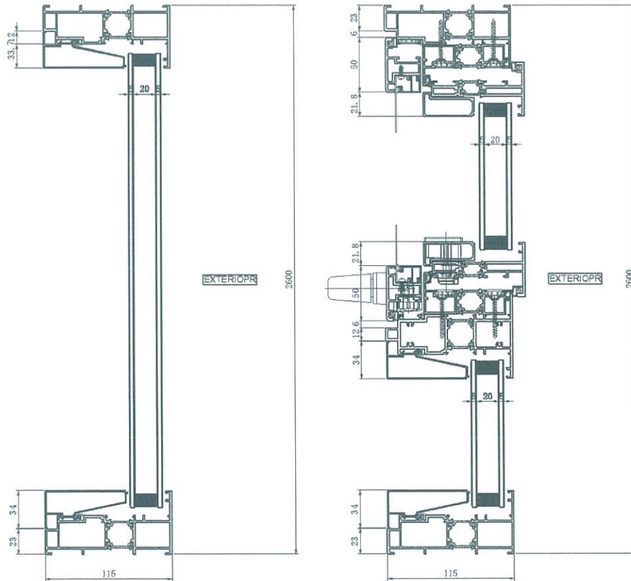
TYPICAL SECTION DETAIL
